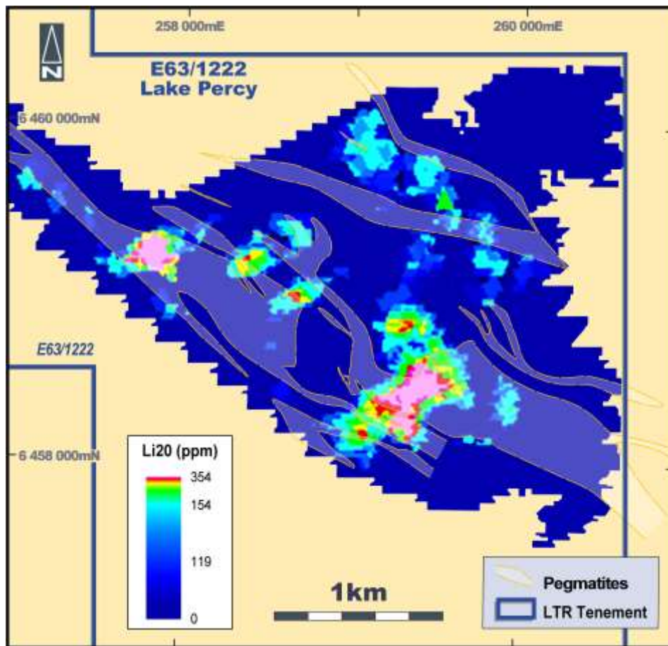
Figure 1: Lake Percy Project – Soil image showing strong lithium anomalism coincident with mapped pegmatites
