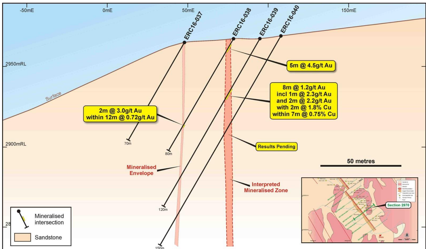
Figure 3: Cross section 2970 showing gold mineralisation intersected in drill holes ERC16-38, ERC16-39 and ERC16-40. Copper mineralisation zone shown as light red zone
