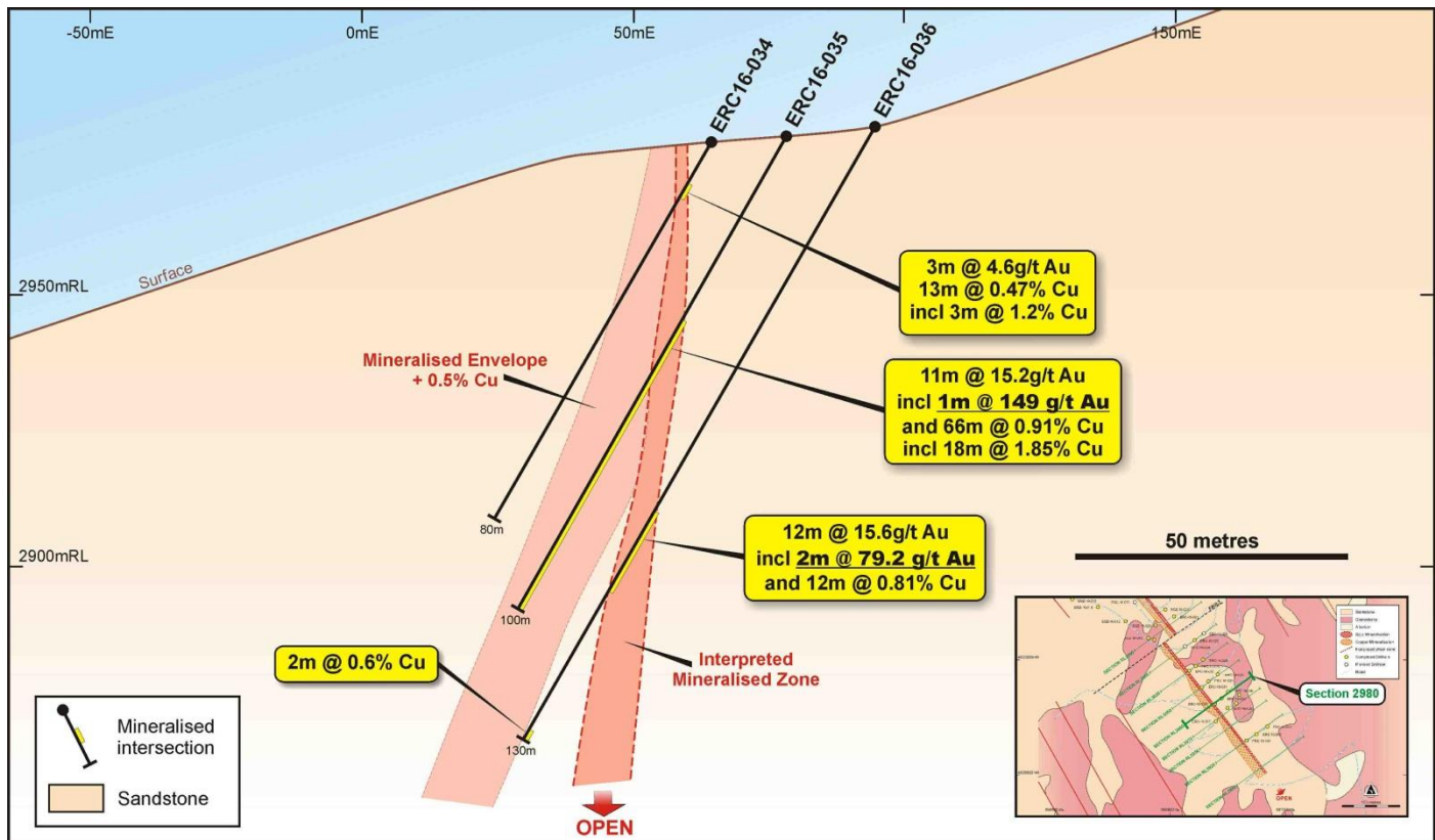
Figure 2: Cross section 2980 showing gold mineralisation intersected in drill holes ERC16-34, ERC16-35 and ERC16-36. Copper mineralisation zone shown as light red zone
