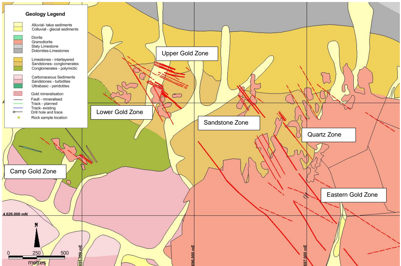
Figure 3: Location map of drilling showing quartz zone and the sandstone zone where visible gold and high grade gold mineralisation is widespread.
