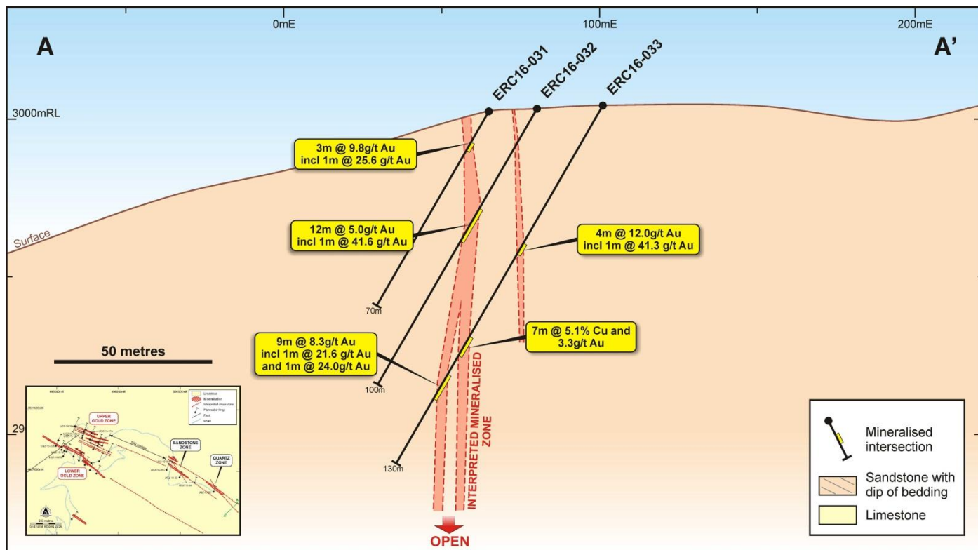
Figure 2: Cross section showing assay results from ERC16-31 to ERC16-33.
