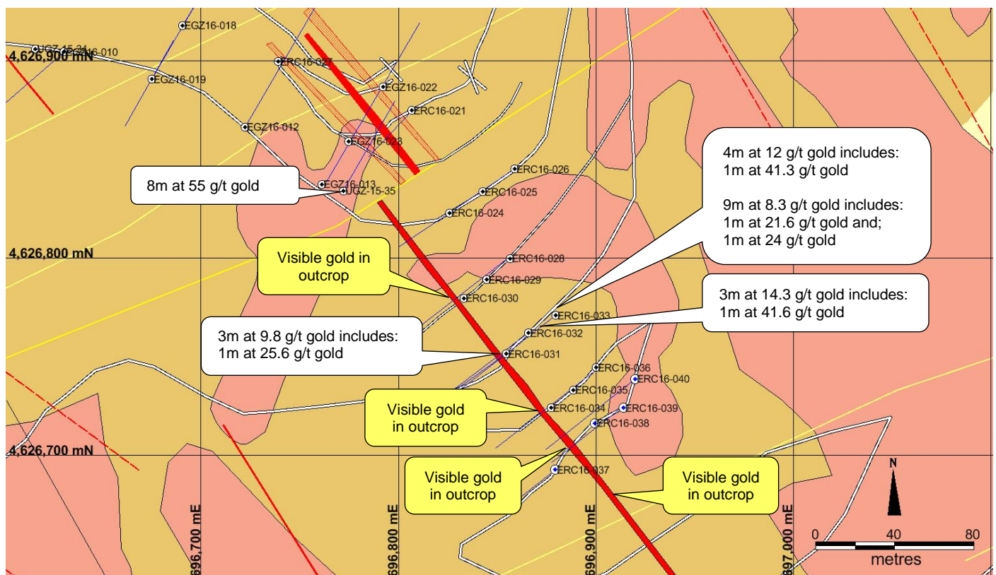
Figure 1: Map showing Quartz Zone and location of outcropping quartz veins (red), drill assay results and planned RC drilling. Tan areas are sandstone, pink areas are granodiorite.
