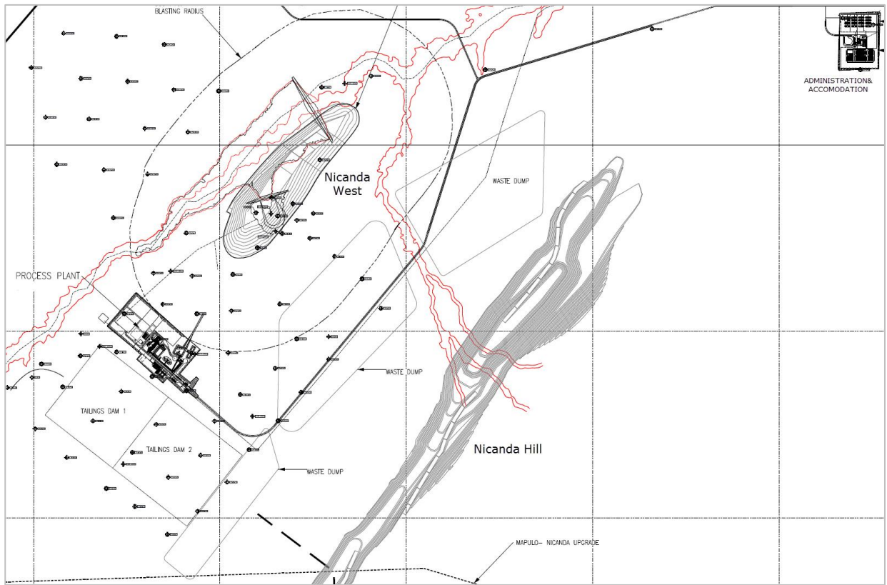
Figure 1 : Revised Site Plan Layout – Balama North
