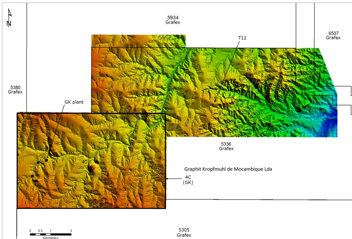
Figure 3: Ancuabe regional topographic surface generated from LIDAR data
