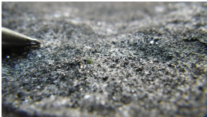
Close up image of diamond drill core from Nicanda Hill prospect.
