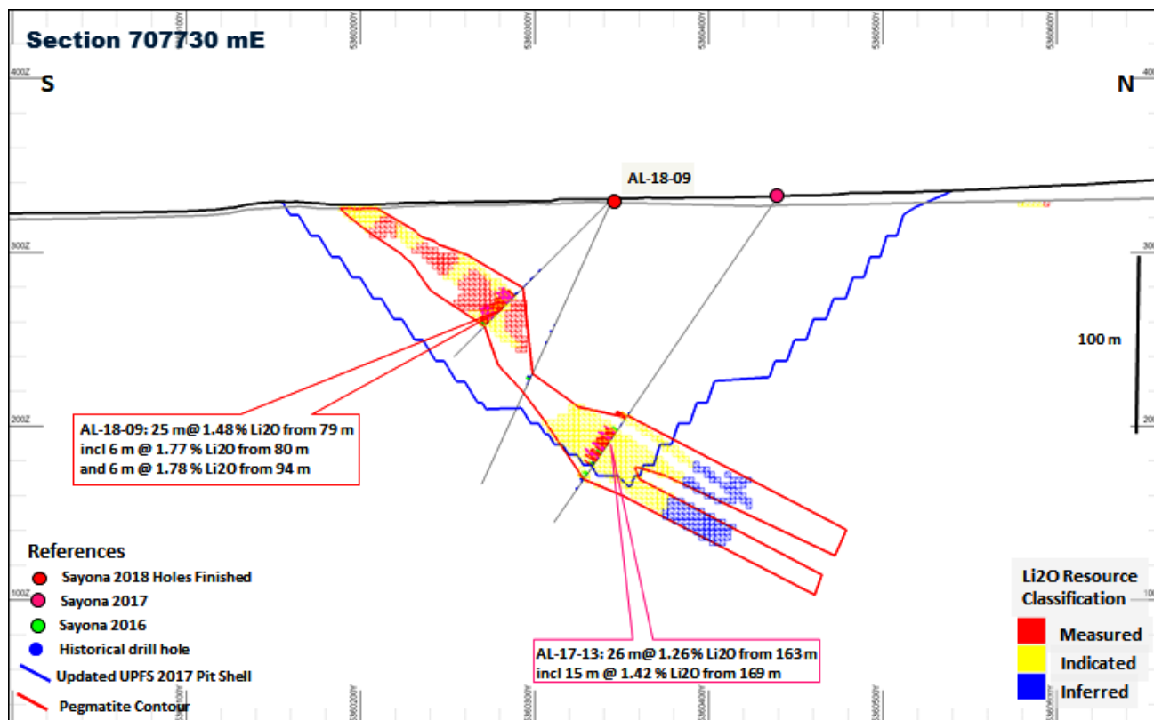
Figure 6: Updated lithium resource classification block model with pit contour from PFS December 2017 for section 707730 mE in the East part of Authier main pegmatite where hole AL-18-09 filled a gap on the resource at mid to shallow levels of the main Authier pegmatite.
