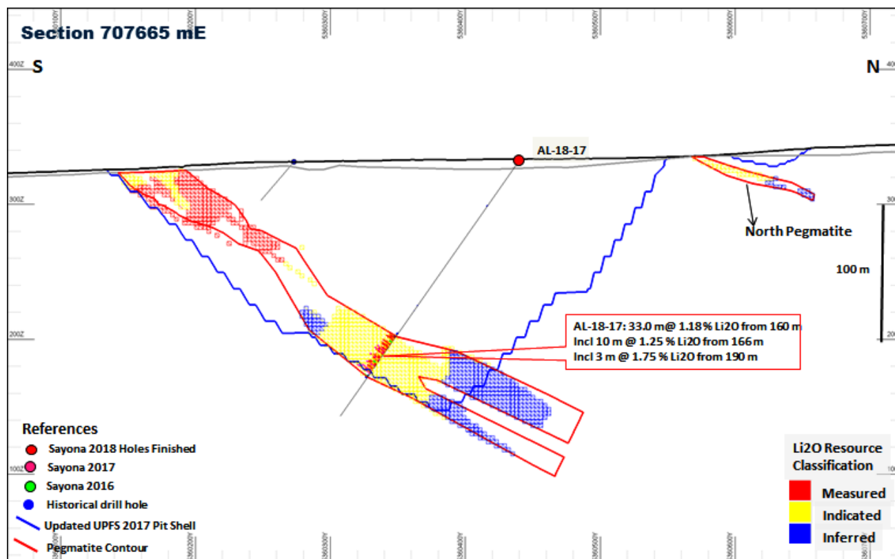
Figure 5: Updated lithium resource classification block model with pit contour from PFS December 2017 for section 707665 in the East part of Authier main pegmatite.
