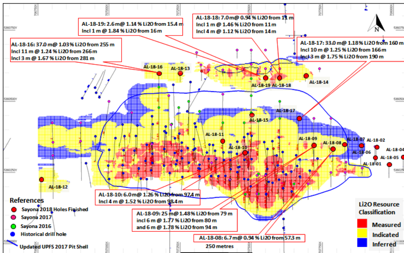
Figure 1: Drill hole collar location plan, updated resource classification block model, pit contour at 300 m RL (PFS 11 December 2017) and significant intercepts from the 2018 drilling.
