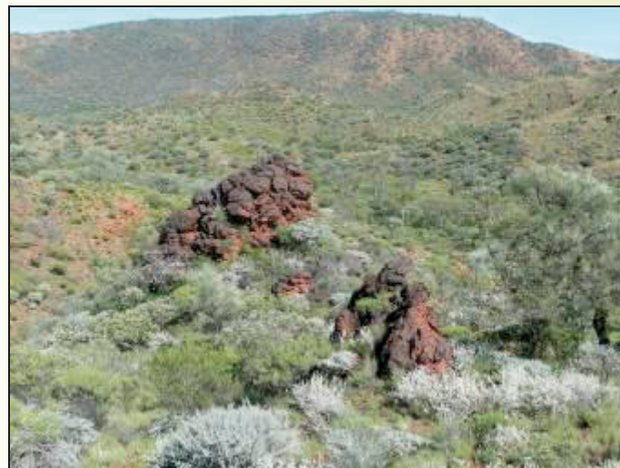
Figure 13: The Black Knob iron outcrop at Tommys Gap.
