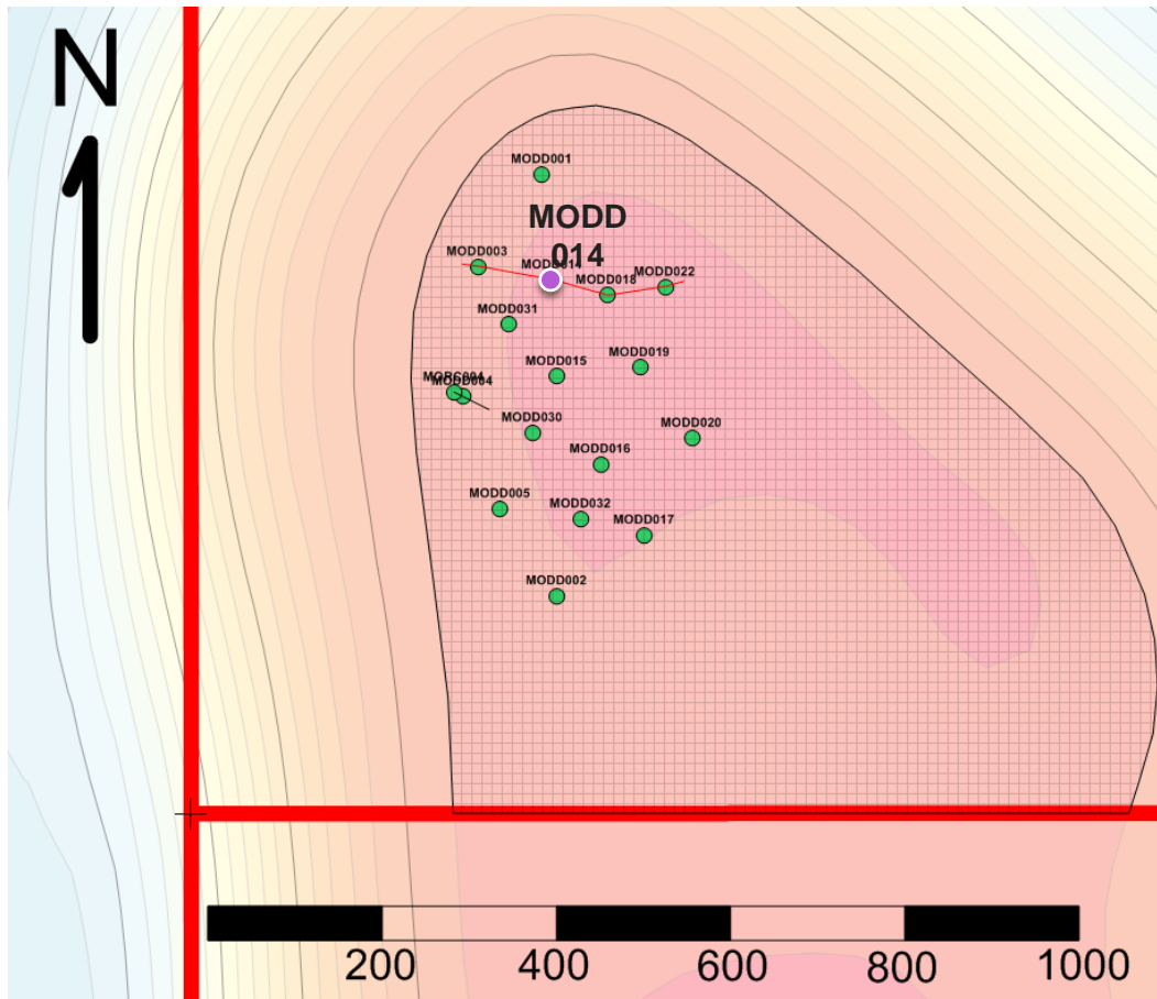
Figure 1. Mustang's Caula Graphite & Vanadium Project, regional geological map depicting the graphitic schist strike through the exploration concessions
