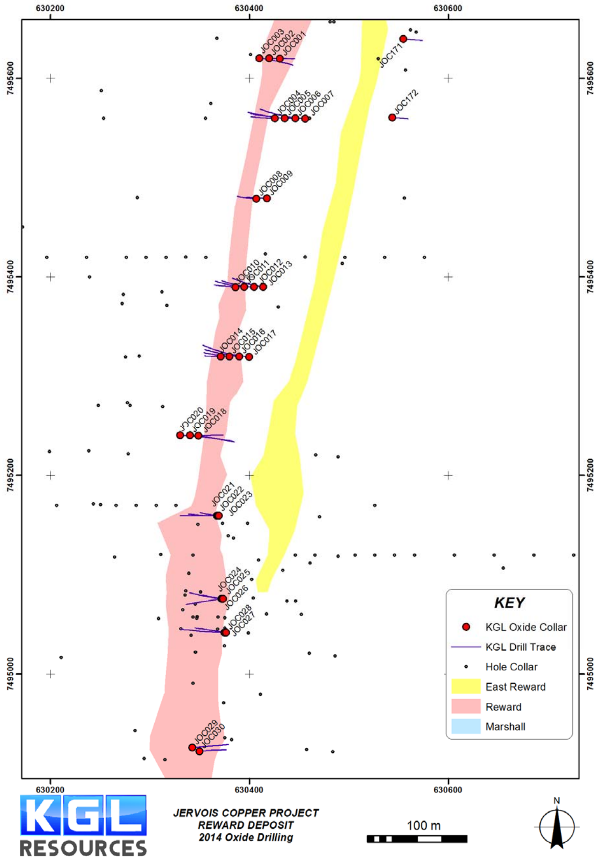
Figure 3 Plan of Reward & East Reward mineralised wireframes, oxide drill collar and drill hole trace
