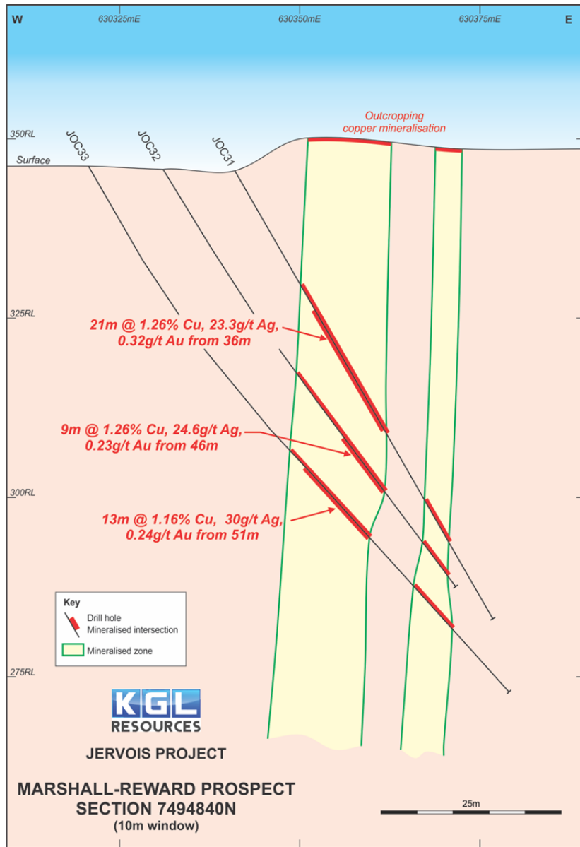
Figure 1 Section 7494840N
