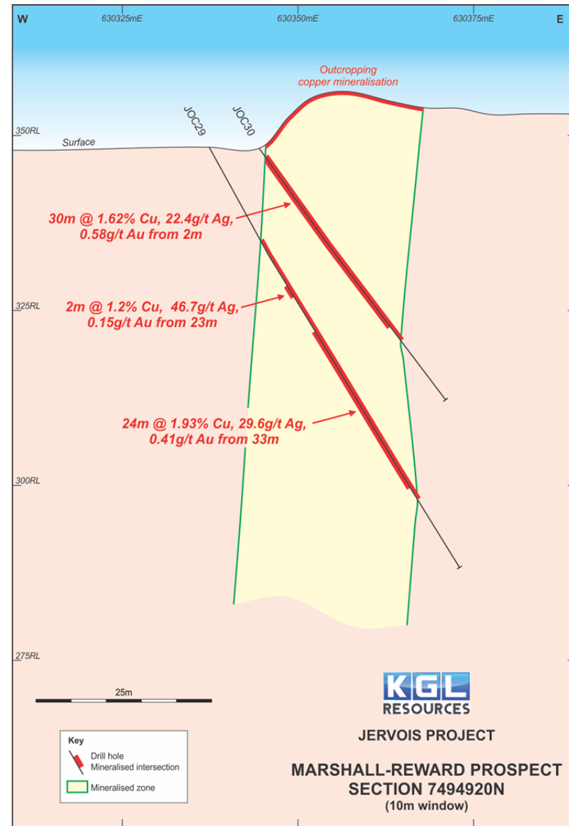
Figure 2 Section 7494920N
