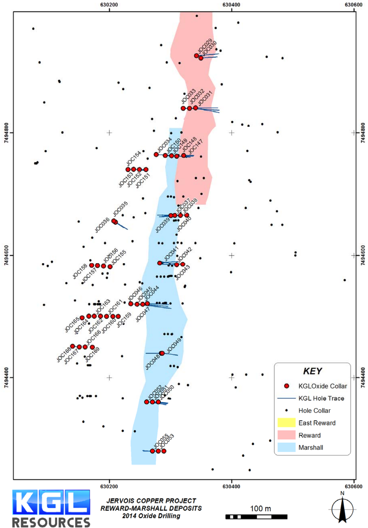
Figure 4 Plan of Marshall, Reward mineralised wireframes, oxide drill collar and drill hole trace
