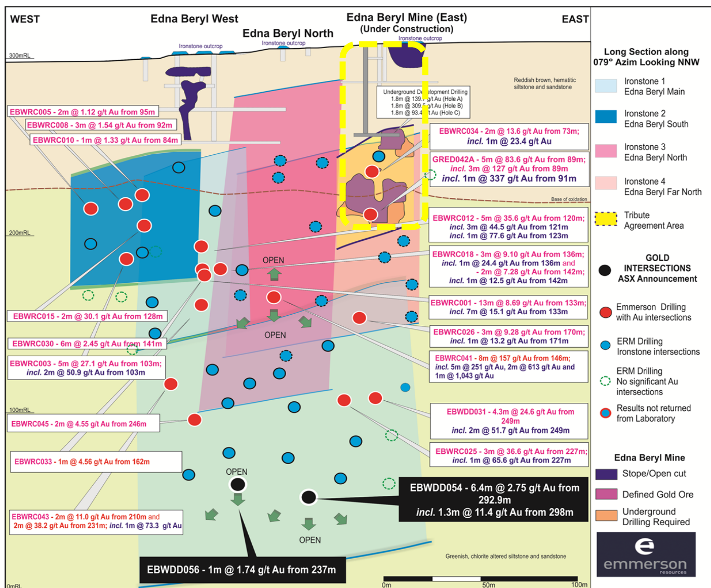
Figure 3: Long section of the Edna Beryl Project - showing 2016 drilling and the Edna Beryl East “small mine” development and tribute area (yellow dotted outline)
