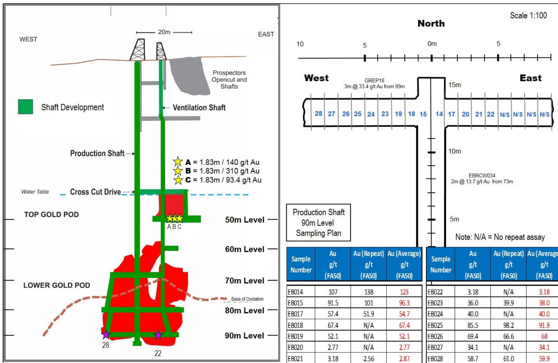
Figure 4: Section of the Edna Beryl Underground Development within the Tribute Area (yellow outline in fig 2). Also development drive and assay results from the 90m Level.
