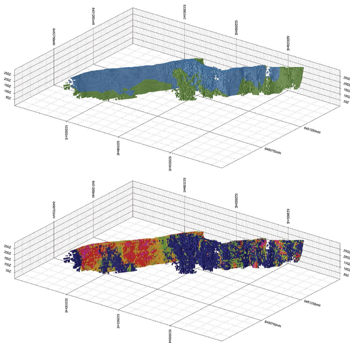
Figure 6. Railway Mineral Resource - block model looking northwest illustrating block distribution by resource classification (top) and cobalt grade (bottom).
