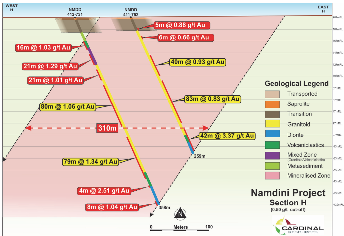
Figure 2: Diamond Drill Holes NMDD413-731 and NMDD411-752 with mineralised zone of 310m
