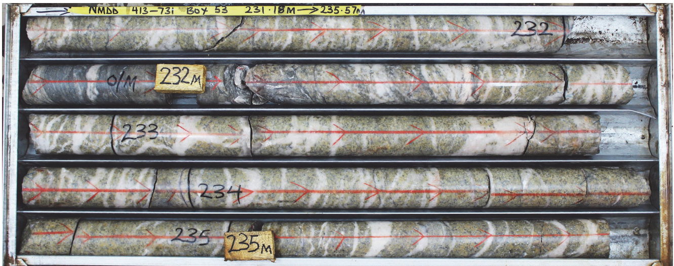
Figure 4: Mineralised granitoid with quartz veining within 79m @ 1.34 g/t Au zone (NMDD413-731)
