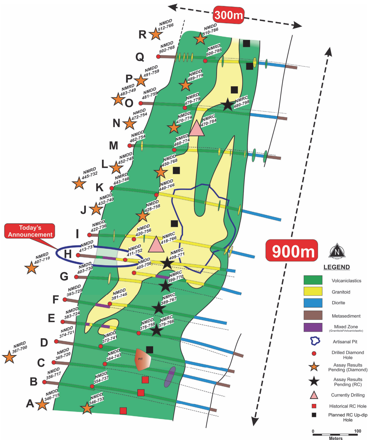
Figure 1: Location of diamond drill holes NMDD413-731 and NMDD411-752
