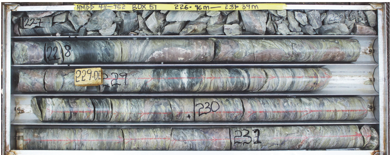
Figure 5: Mineralised volcanoclastics with quartz veining within 42m @ 3.37 g/t Au zone (NMDD411-752)
