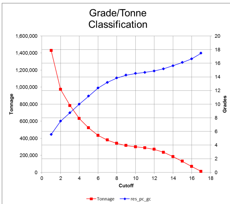
Figure 0-2 Tonnage and grade graph of combined Indicated and Inferred Resources.
