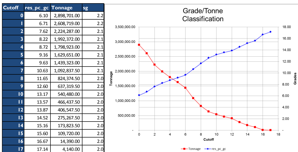
Figure 0-2: Tonnage and grade graph of combined Measured, Indicated and Inferred
