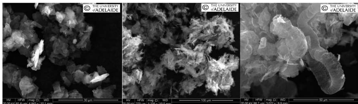
Plate 4. SEM images of Archer Campoona graphite flakes (92% TGC) (left) used for preparation of chemical and electrochemical prepared intercalated graphite microparticles (middle and right)
