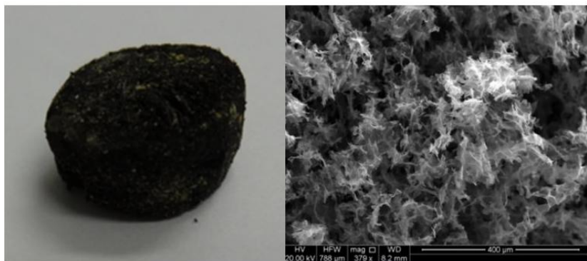
Graphene aerogel from raw graphite
