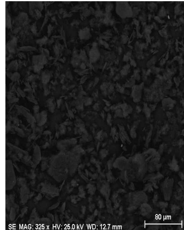
Bulk flotation re-cleaner concentrates + tail under SEM
