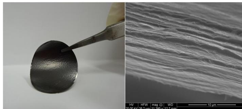
Membrane of graphene sheets from raw graphite
