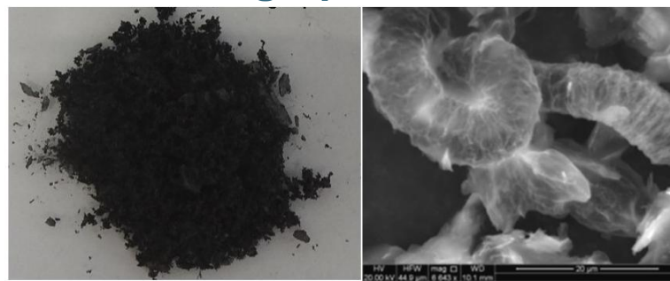
Thermally intercalated graphite from medium-grade 92%C Campoona concentrate
