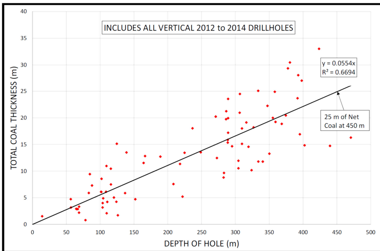
Net Coal Calculations for 2012-2014 Drilling (Vertical Holes Only)
