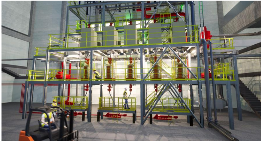
Figure 5 – Front end section of Silumina Anodes™ plant design
