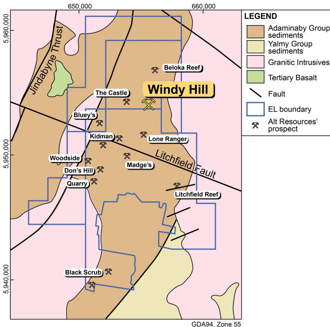
Figure 1. Location of the Paupong Project, showing Windy Hill and the distribution of other prospects within the licence area. The geology shown is based on the 1:250,000 Bega-Mallacoota map sheet.
