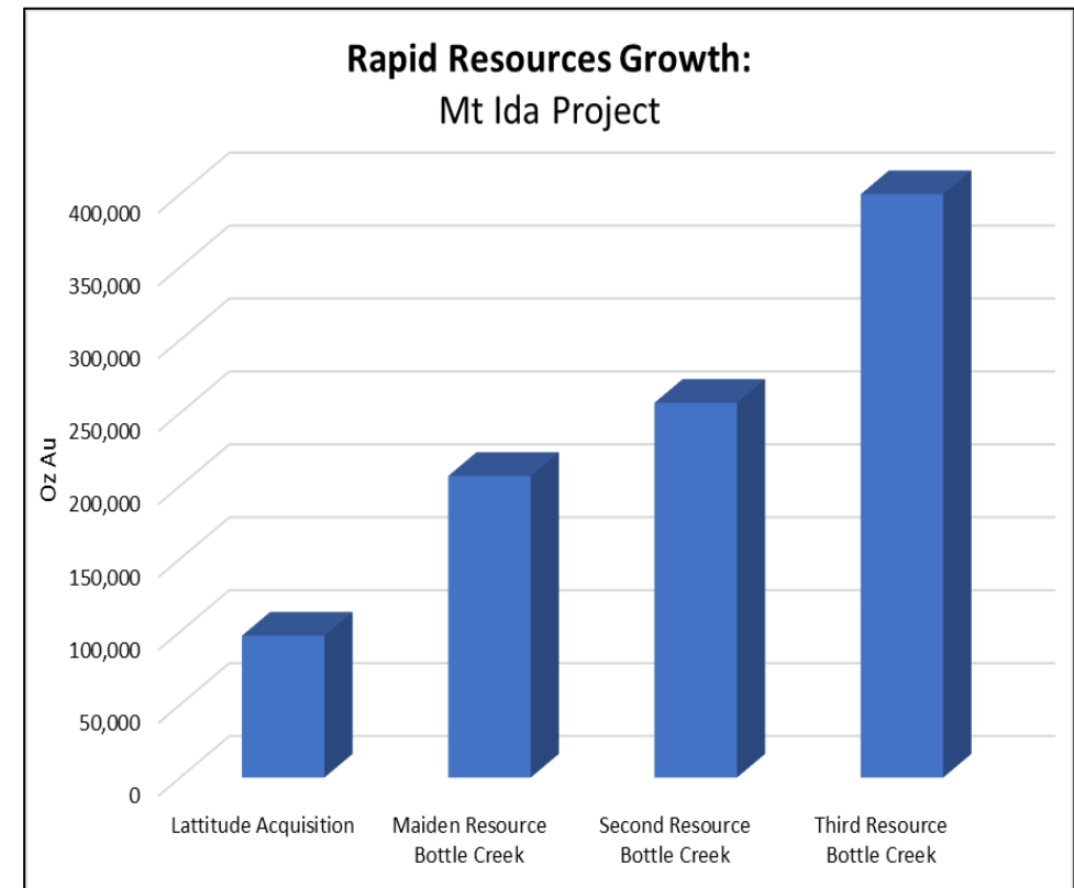
Graph showing Resource growth at Alt's Mt Ida Project.
