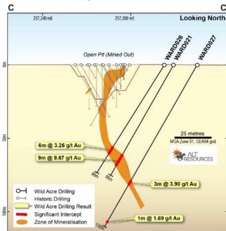
QUINNS PROJECT Boudie Rat Prospect Oblique Section - Open Pit
