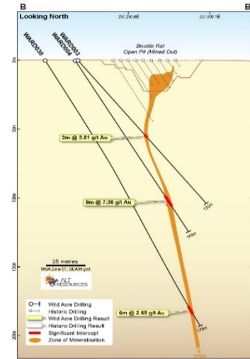
QUINNS PROJECT Boudie Rat Prospect Oblique Section - Open Pit
