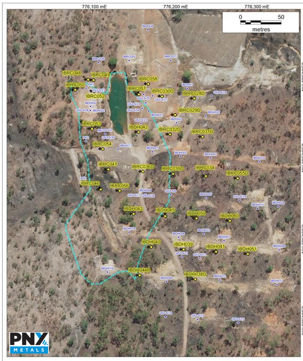
Figure 2: Iron Blow drill collar plan on aerial photograph with blue hashed line representing the outline of the resource projected to surface
