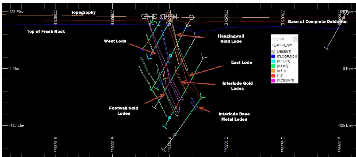
Figure 1: Section showing modelled mineralisation envelopes (CSA Global)
