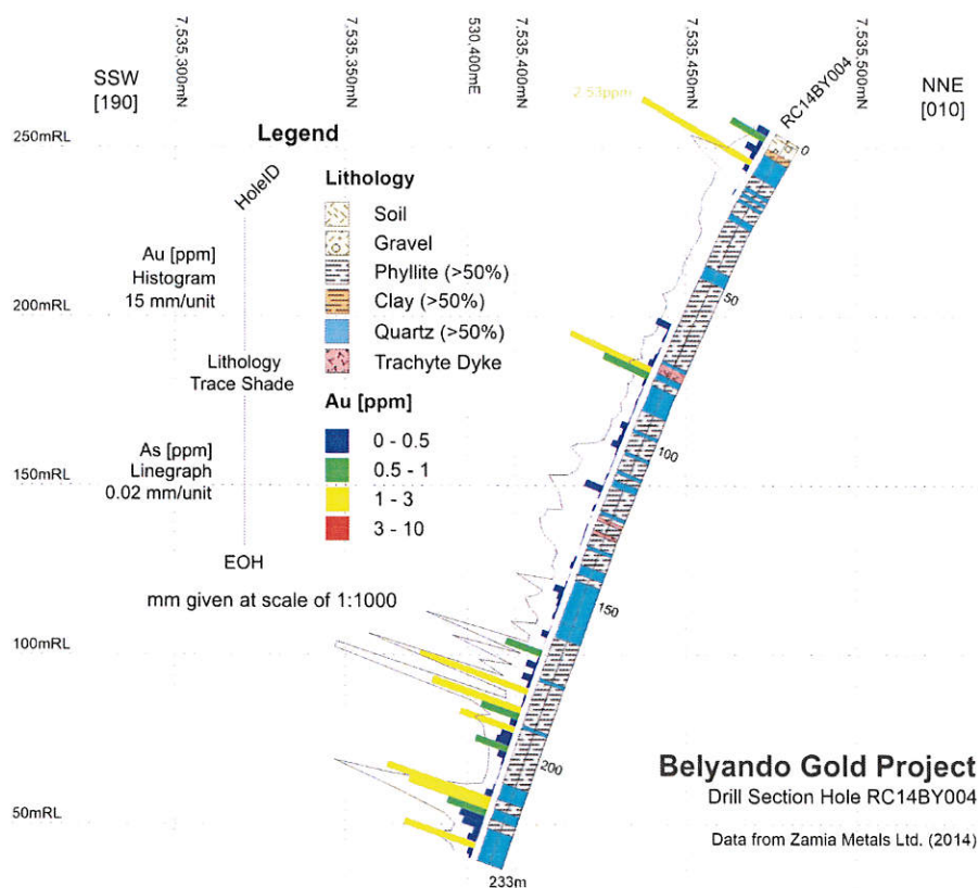
Figure 5. Drill section of hole RC14BY004, showing a graphical representation of gold ('Au') and arsenic ('As') assays. Coordinates given are MGA94, Zone 55S.
