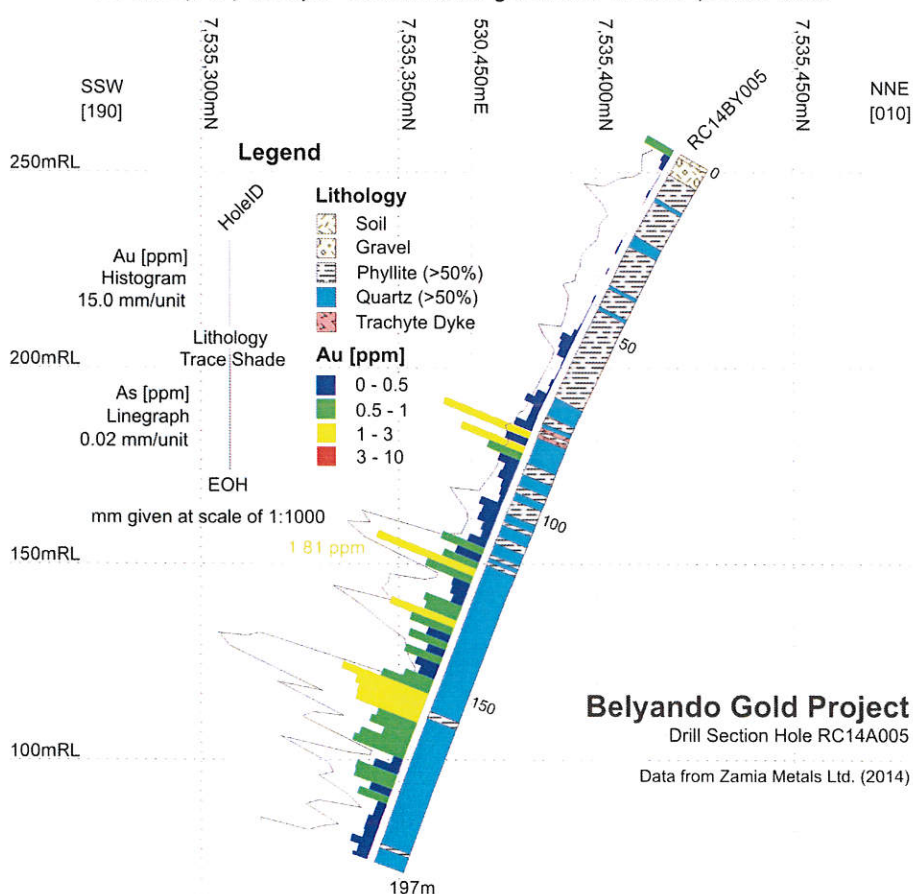
Figure 6. Drill section of hole RC14BY005, showing a graphical representation of gold ('Au') and arsenic ('As') assays. Coordinates given are MGA94, Zone 55S.
